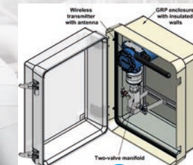
GRP structures provide benign environments for wireless-enabled instruments - extending applications potential in highly automated processing plants. They allow antennas to remain inside the enclosure.
