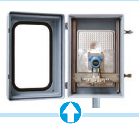
Two-part enclosures are easy to panel mount, with tube entry via top or base. MULTIBOX has thick and shallow sections, either of which can be used as the door. 12 sizes.
