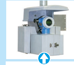
Two-part MESC enclosure meeting Shell standards, with flaps for manifold operation.
