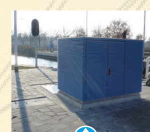
Multi-compartment cabinet houses the electronics and hydraulic systems controlling a waterway lock. Decorative cladding makes the structure an attractive asset to support leisure use.
